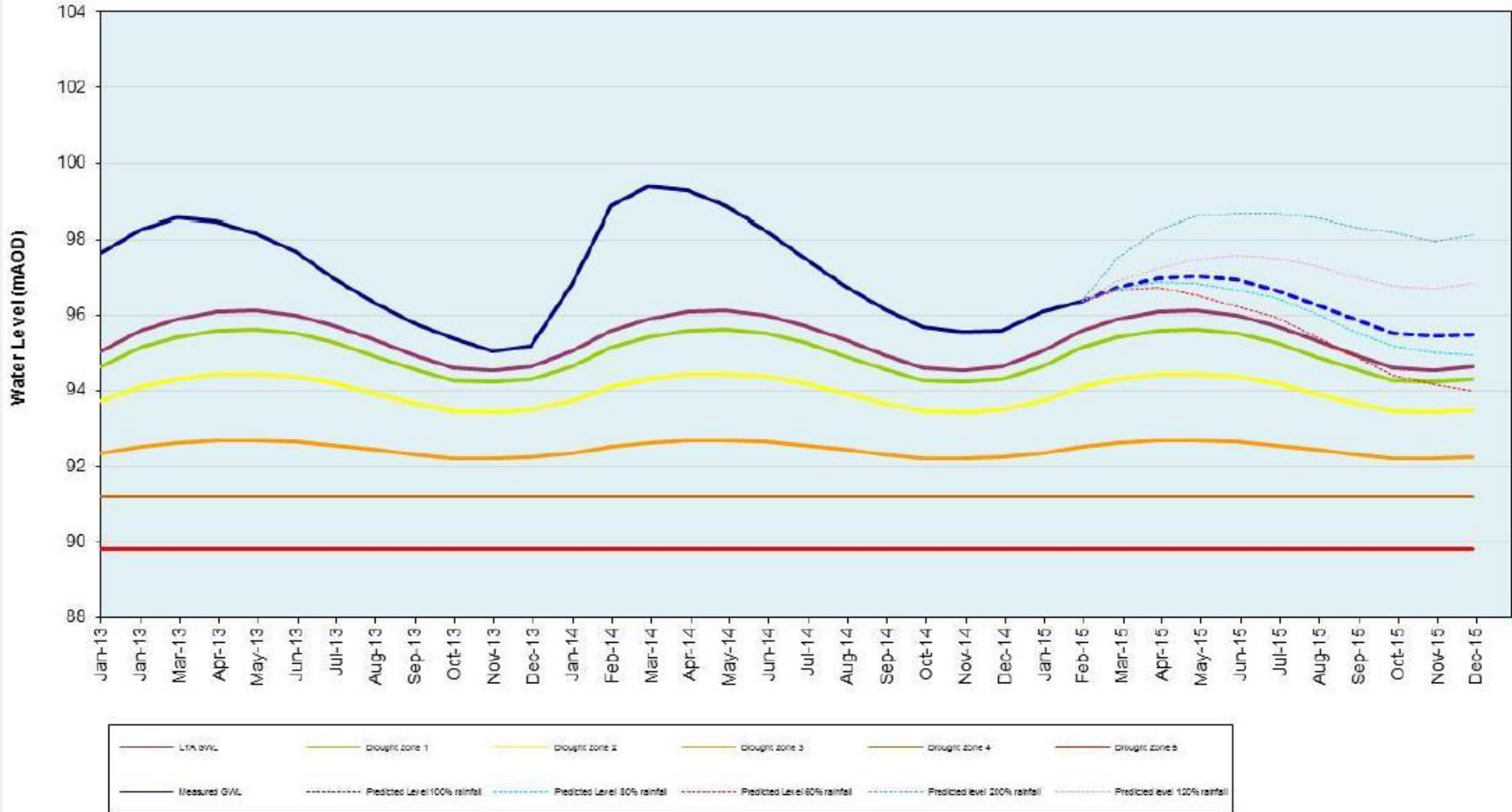
AW Central Region Groundwater Drought Triggers into 2015
